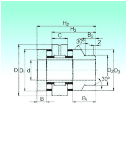
ZARN 1747 L TN Bearing 2D drawings and 3D CAD models
