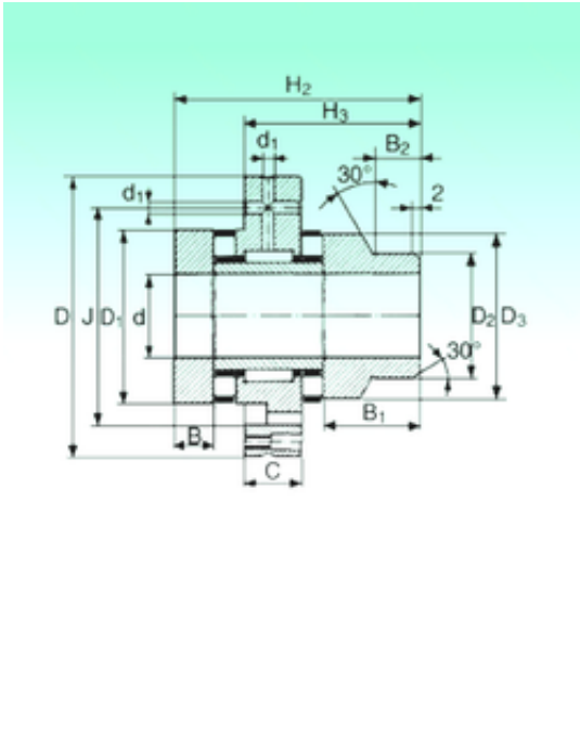
ZARF 1762 L TN Bearing 2D drawings and 3D CAD models
